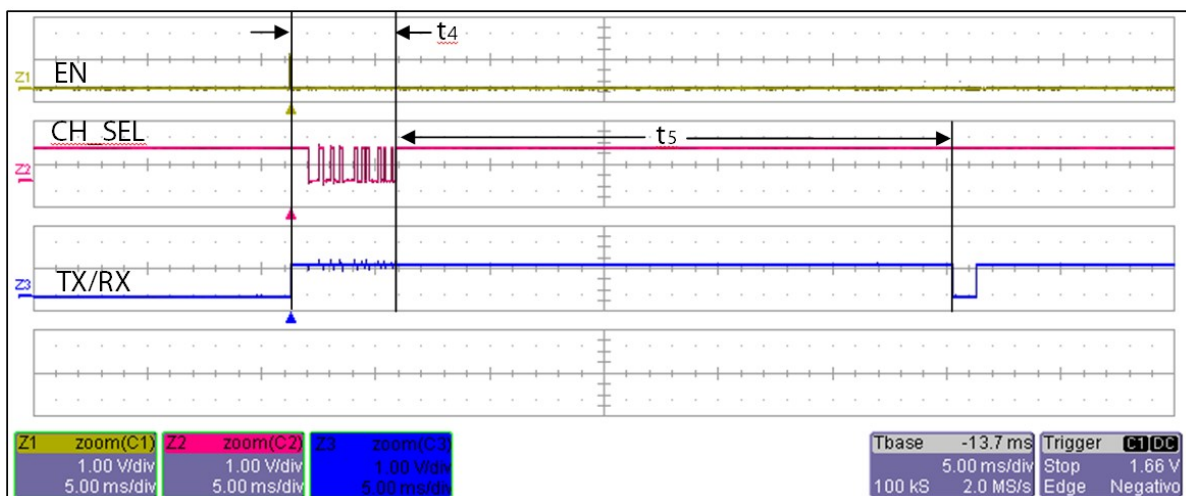
Figure 3: timings. t 4 < 90 ms; t 5 = 20 ms typ.
